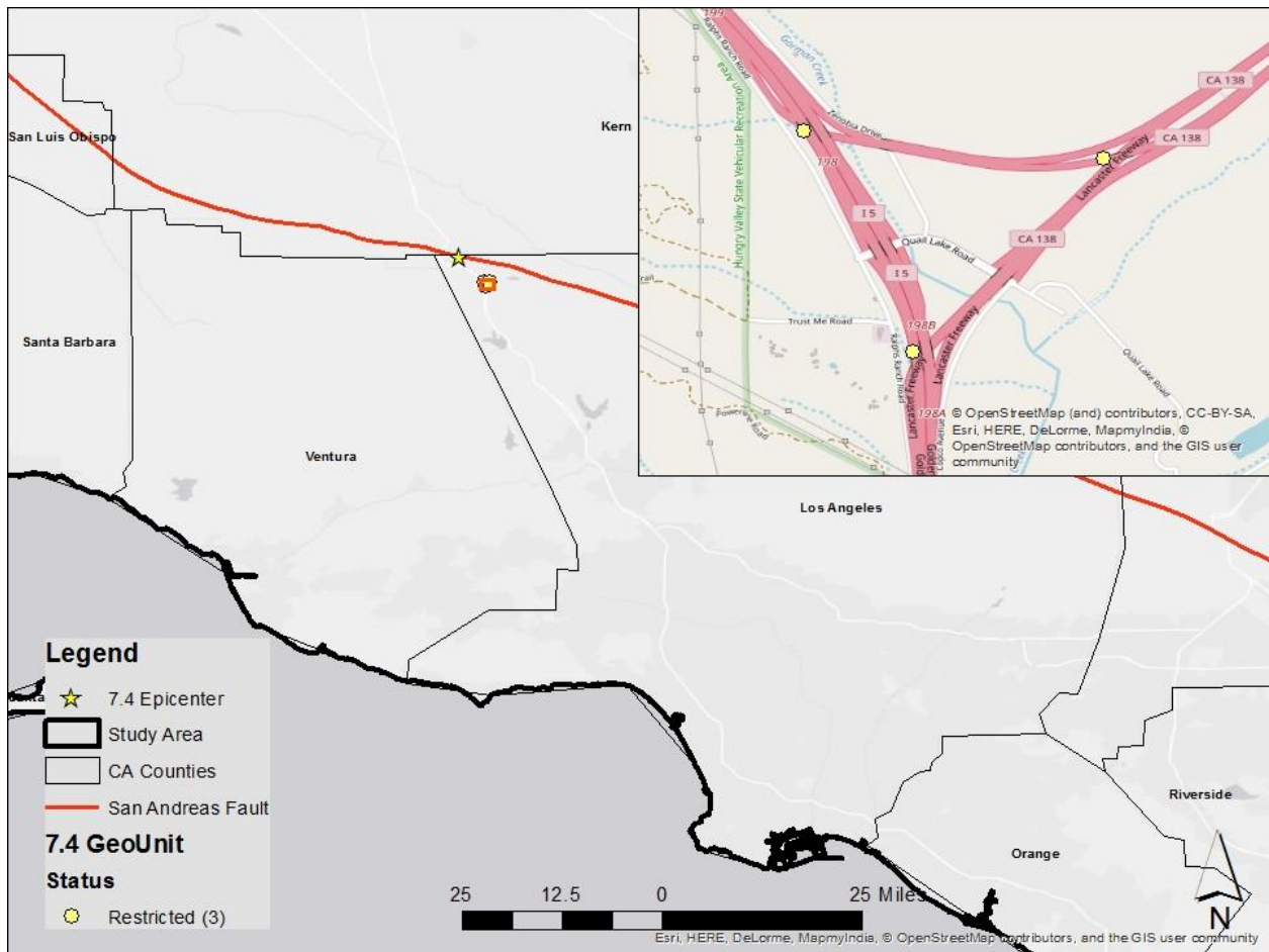
Figure 25 M7.4 Geological Unit Restrictions and Closures (Point Counts in Parenthesis)
